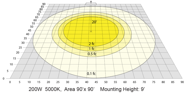
200W 5000K, Area 90'x 90' Mounting Height: 9'
