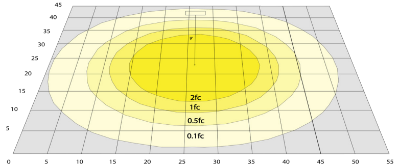
40W 5000K, Area 45'x 55' Mounting Height: 9'
