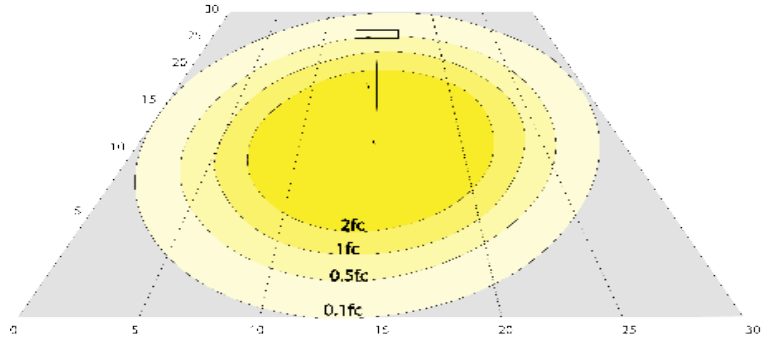
25W 3000K, Area 30'x 30' Mounting Height: 9'
