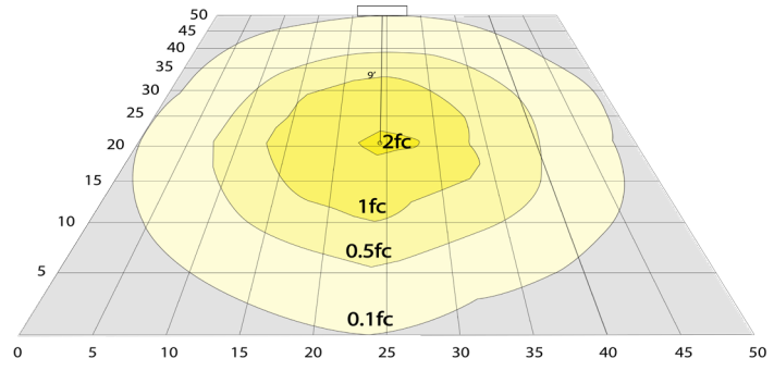
18W, 5000K Area 50'x 50' Mounting Height: 9'
